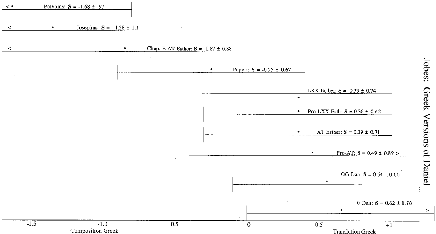
Graph 3: S-Numbers with Standard Deviations
