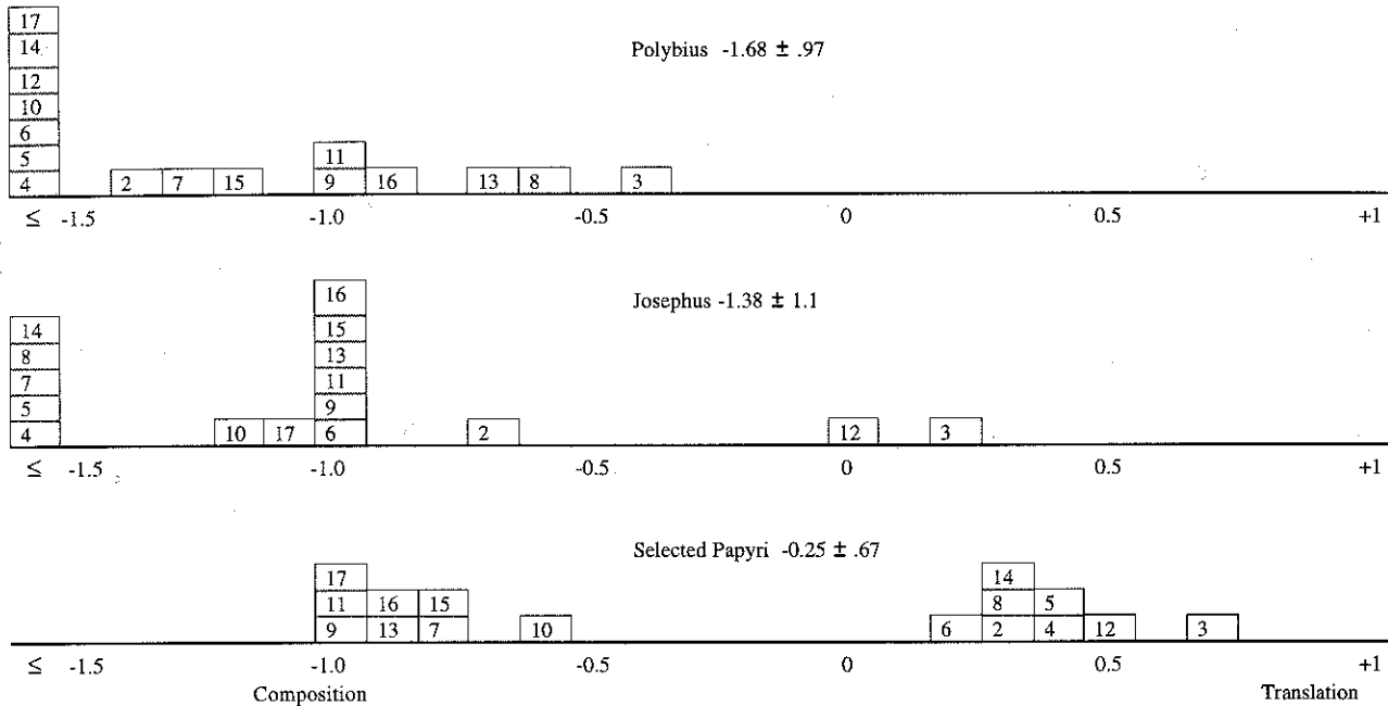
Graph 2: A Profile of the Syntax of Texts Composed in Greek
